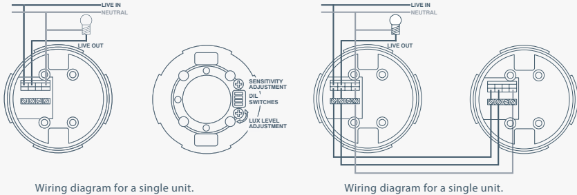
Wiring diagram for a single unit.
